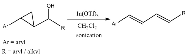
Scheme 1. Rearrangement of cyclopropyl carbinols.
